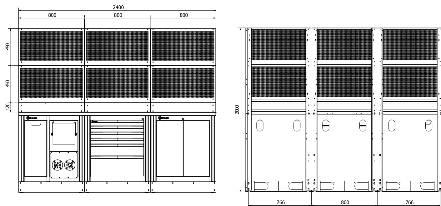
CONFIGURAZIONE 2400 CON PANNELLI FORATI CONFIGURATION 2400 WITH PERFORATED PANELS COD. 3DP99W14IFV
