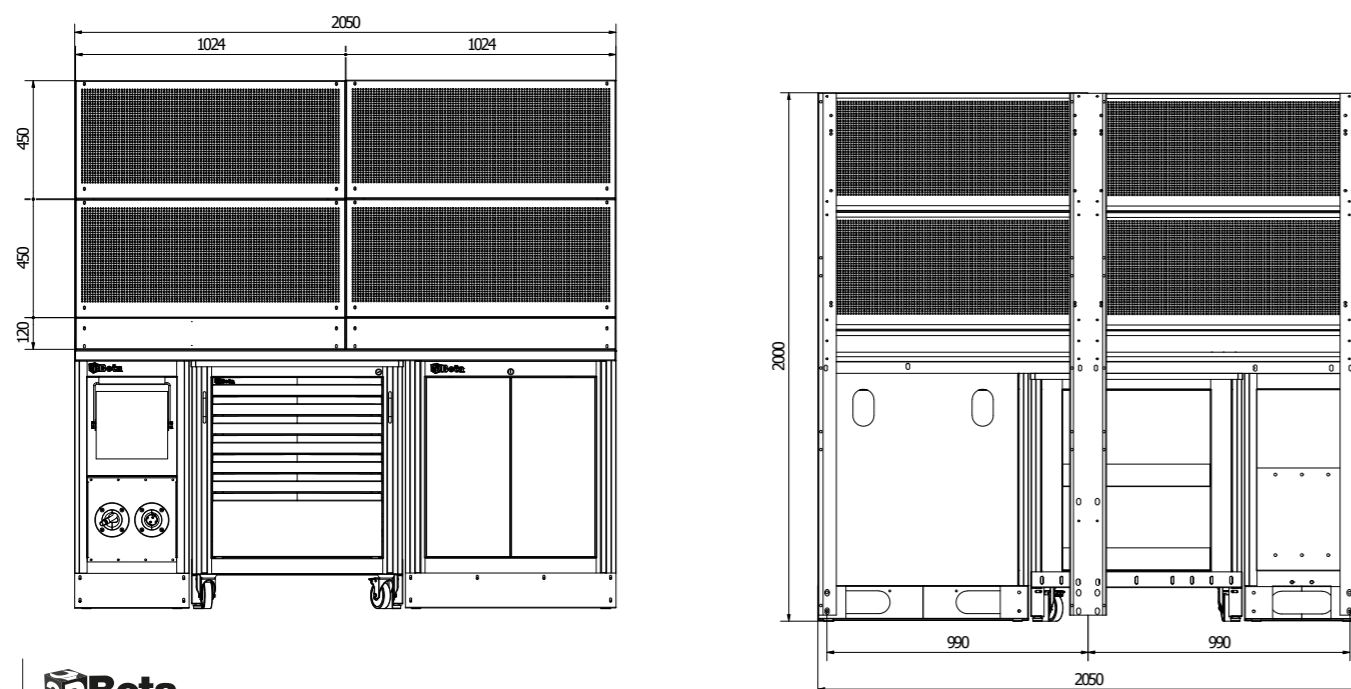
CONFIGURAZIONE 2050 CON PANNELLI FORATI CONFIGURATION 2050 WITH PERFORATED PANELS COD. 3DP99W11IFU
