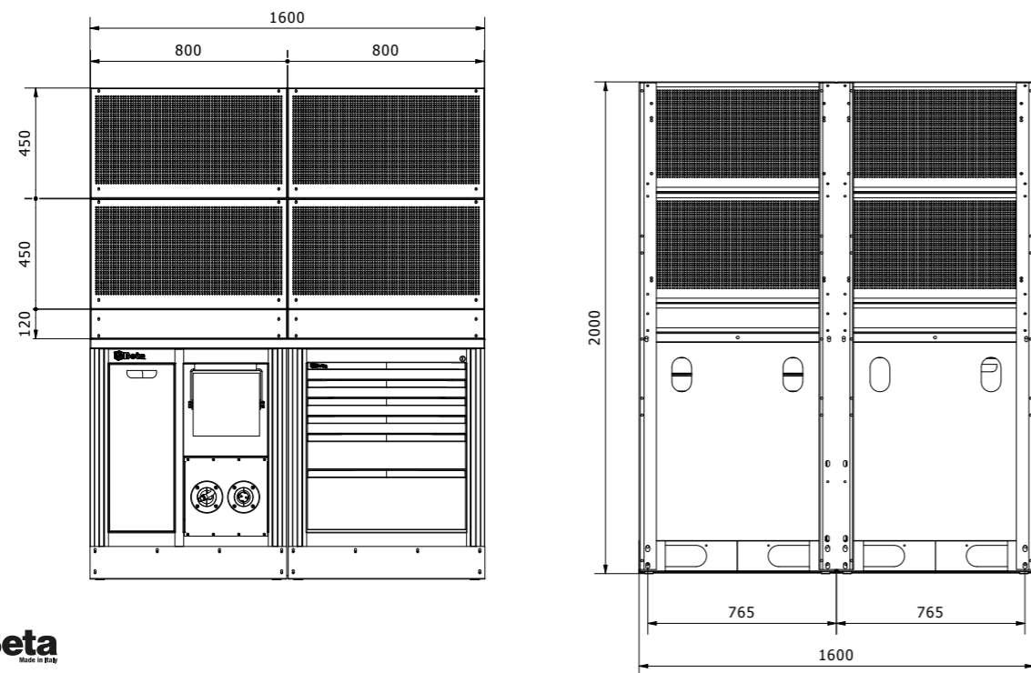
CONFIGURAZIONE 1600 CON PANNELLI FORATI CONFIGURATION 1600 WITH PERFORATED PANELS COD. 3DP99W06IFT
