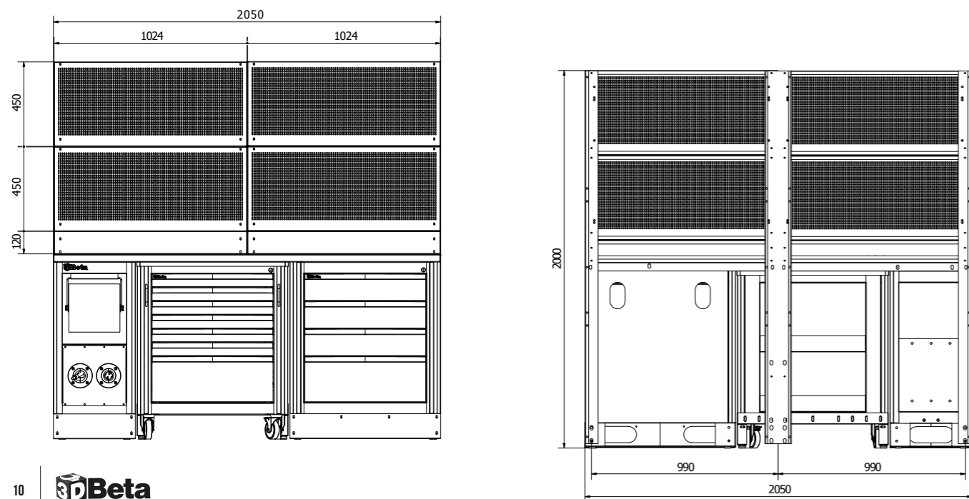
CONFIGURAZIONE 2050 CON PANNELLI FORATI CONFIGURATION 2050 WITH PERFORATED PANELS COD. 3DP99W08IFU
