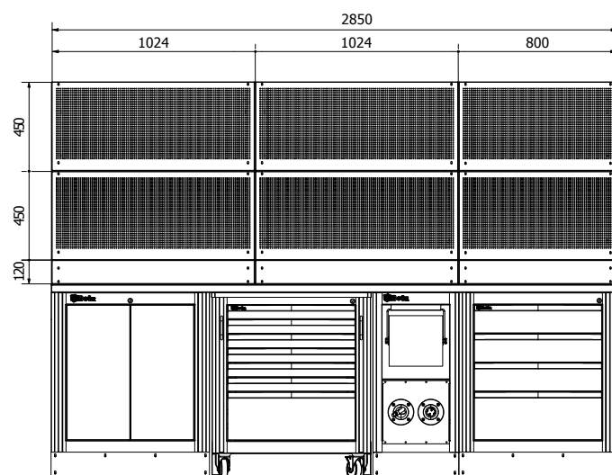
CONFIGURAZIONE 2850 CON PANNELLI FORATI CONFIGURATION 2850 WITH PERFORATED PANELS COD. 3DP99W16IFW
