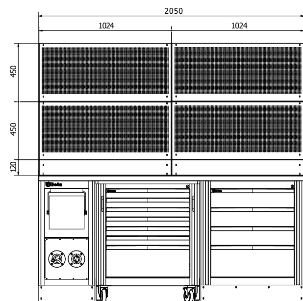
CONFIGURAZIONE 2050 CON PANNELLI FORATI CONFIGURATION 2050 WITH PERFORATED PANELS COD. 3DP99W08IFU
