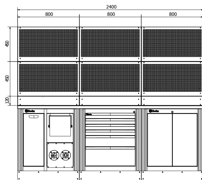
CONFIGURAZIONE 2400 CON PANNELLI FORATI CONFIGURATION 2400 WITH PERFORATED PANELS COD. 3DP99W14IFV
