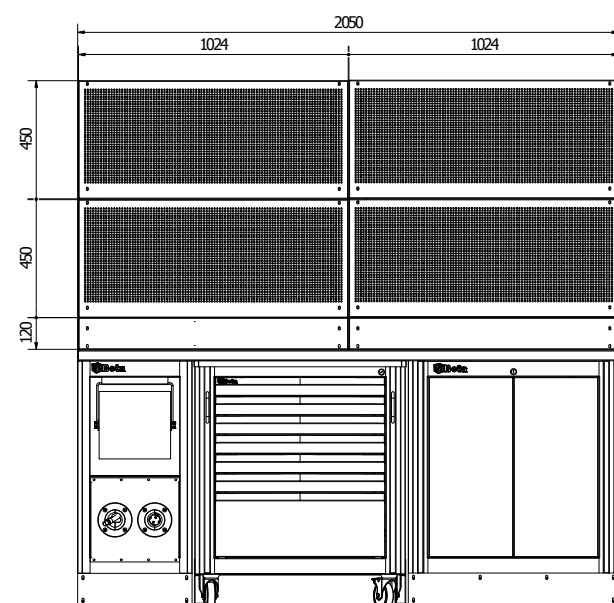
CONFIGURAZIONE 2050 CON PANNELLI FORATI CONFIGURATION 2050 WITH PERFORATED PANELS COD. 3DP99W11IFU
