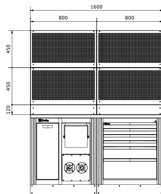
CONFIGURAZIONE 1600 CON PANNELLI FORATI CONFIGURATION 1600 WITH PERFORATED PANELS COD. 3DP99W06IFT
