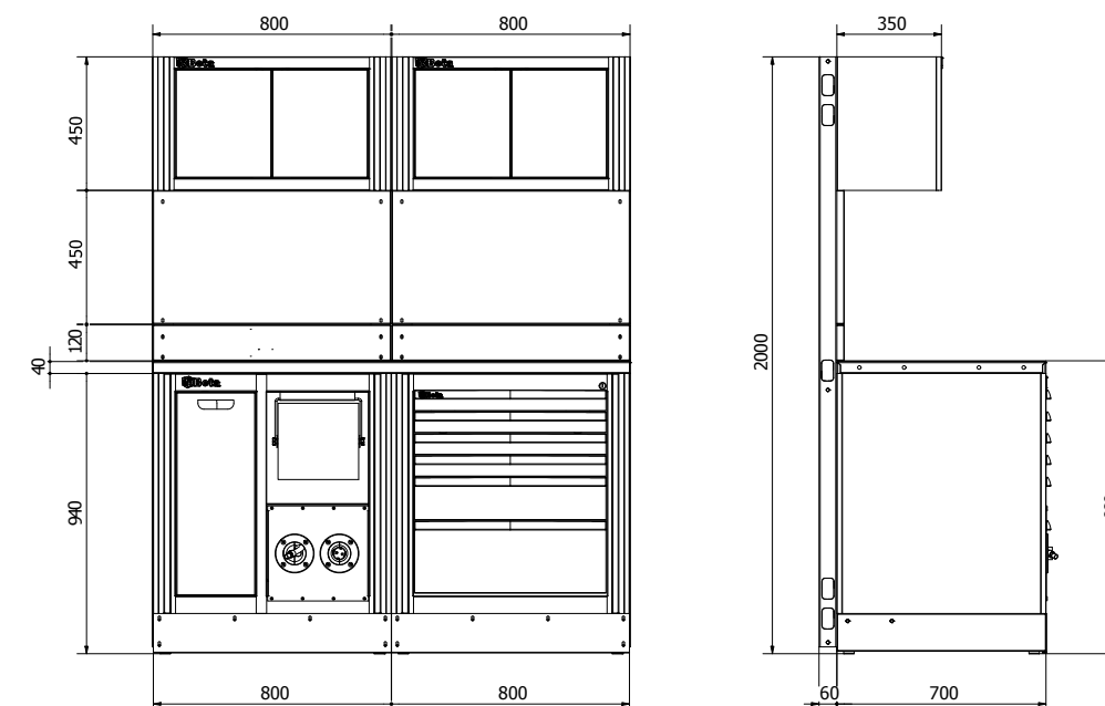
CONFIGURAZIONE 1600 CON PENSILI A DUE ANTE CONFIGURATION 1600 WITH TWO-DOOR WALL CABINETS COD. 3DP99W05IFT
